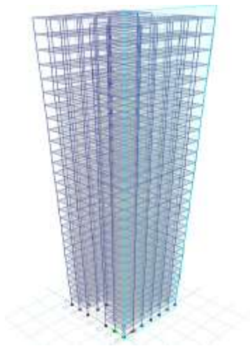
Figure 10 Isometric View of RC Frame
