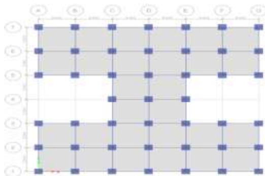
Figure 2 Plan of RC Frame model
