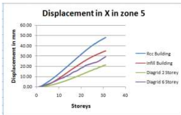
Figure 14 Displacements in X-direction
