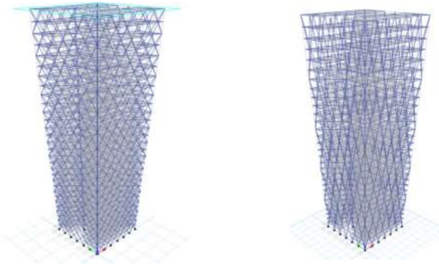
Figure 12 Isometric View of diagrid 2 storey model Figure 13 Isometric View of diagrid 6 storey model
