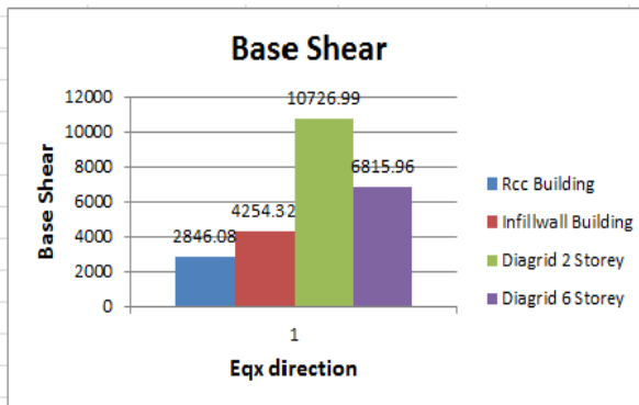
Figure 21 Base Shear in X-direction.
