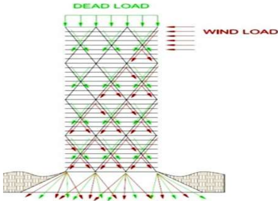
Figure 1 Load Distribution in Diagrid Structural System.
