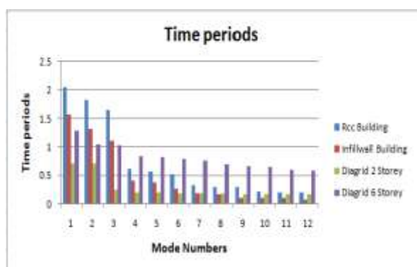
Figure 20. Time Period in X-direction
