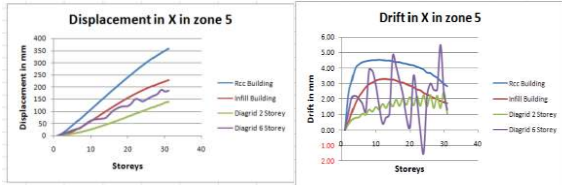
Figure 16 RS Displacements in X-direction Figure 17 RS Drifts in X-direction
