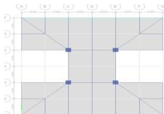
Figure 5 Plan of diagrid 6storey model
