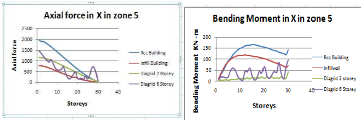
Figure 18. Axial Forces in X-direction
